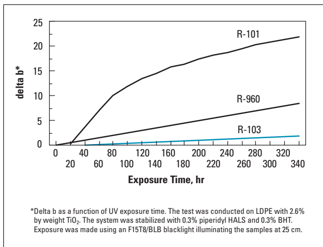
Figure 3. Ti-Pure™ R-103 Discoloration Resistance in HALS Stabilized LDPE
