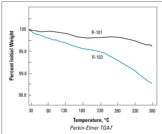
Figure 4. Thermo-Gravimetric Measurement of TiO 2 Volatility
