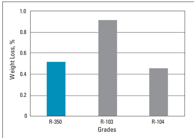
Figure 2. High Temperature Weight Loss
