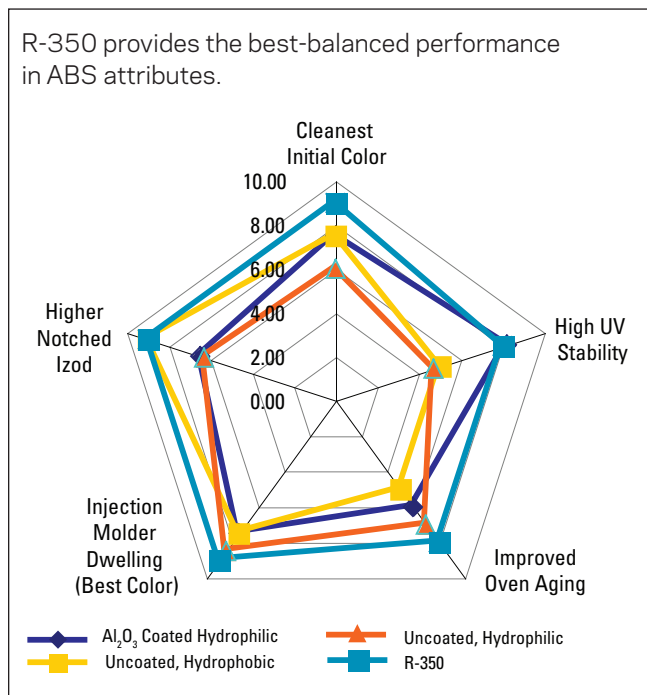
Figure 5. ABS Performance — Summary Data
