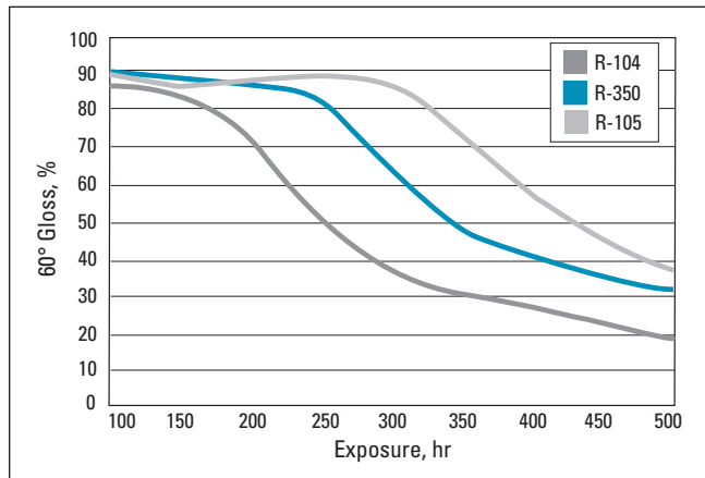
Figure 4. Polyolefin Gloss Retention
