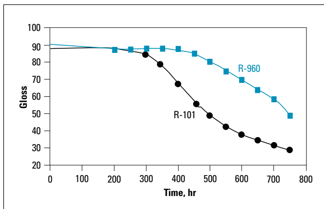
Figure 2. Gloss Retention of Polypropylene, Xenon Exposure
