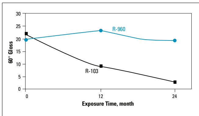
Figure 3. Gloss Retention of PVC, Florida Exposure 45° South
